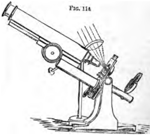
Arrangement of Microscope for Opaque Objects.
